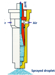
Figure 11: Air induction nozzles
