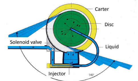
Figure 22: Rotary atomizers
