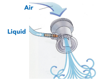
Figure 21: Pneumatic atomizer
