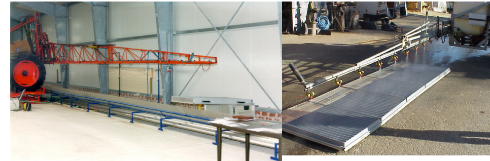
Figure 24: Equipment to measure the quality of the cross distribution of the spray
