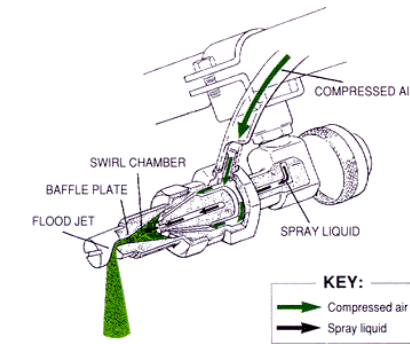
Figure 27: Twin fluid nozzle
